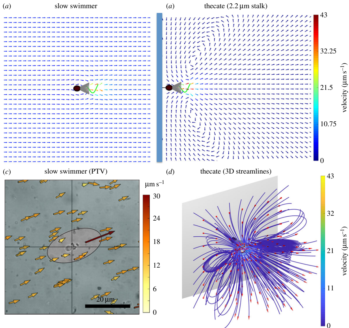
Figure 6. Water flow relative to a choanoflagellate with a collar composed of cylindrical microvilli 5.8 μm long. (a,b) Average velocity vectors calculated relative to a choanoflagellate in the plane of flagellar beating for a slow swimmer (a), and for a thecate cell attached to a wall by a stalk 2.2 μm long (b). Velocities were averaged over one flagellar beat cycle. Size scale: cell body length = 4.4 μm. (c) Velocity vectors relative to a slow swimmer measured using particle-tracking velocimetry (PTV). Videos (Fastek Hi-Spec 1 camera, 100 fps) were made of S. rosetta viewed through a 63x Plan Apo oil immersion lens on a Leica DM 2500 compound microscope with interference contrast illumination. Velocities of 1 μm polystyrene beads relative to the swimming cell were calculated using in-house software written to use Python v. 2.7 bindings to the OpenCV v. 2.4 Computer Vision Library ( https://opencv.org/ ). (d) A three-dimensional image of the streamlines around a simulated thecate cell, noting the toroidal eddies. (Online version in colour.)
